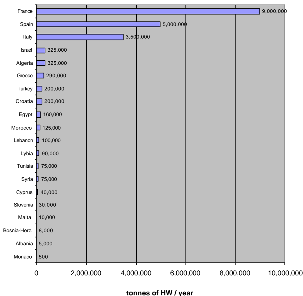
Figure 1.1 Estimated hazardous waste generation in the MAP countries
